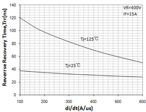
Fig.5 Reverse recovery time versus di/dt
