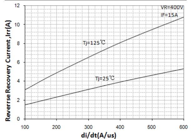
Fig.6 Peak reverse recovery current versus di/dt
